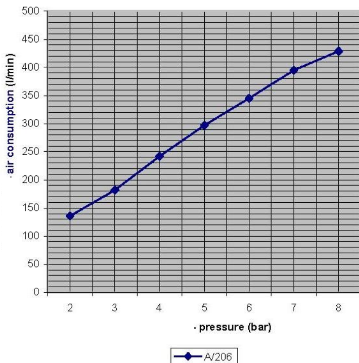
Air consumption graph for A/206
